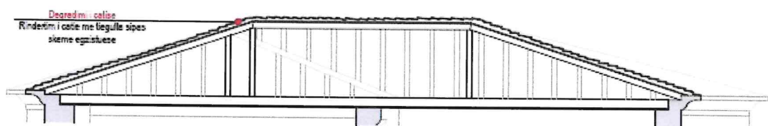
PRERJE CATIE SHK:1:50
